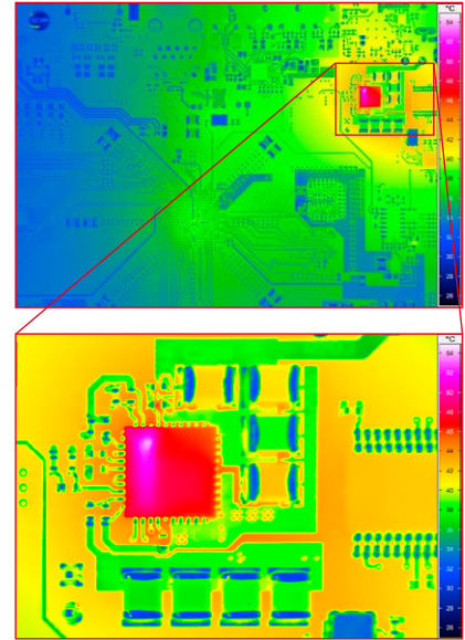
Format-filling image of circuit board and detailed zoom into image
